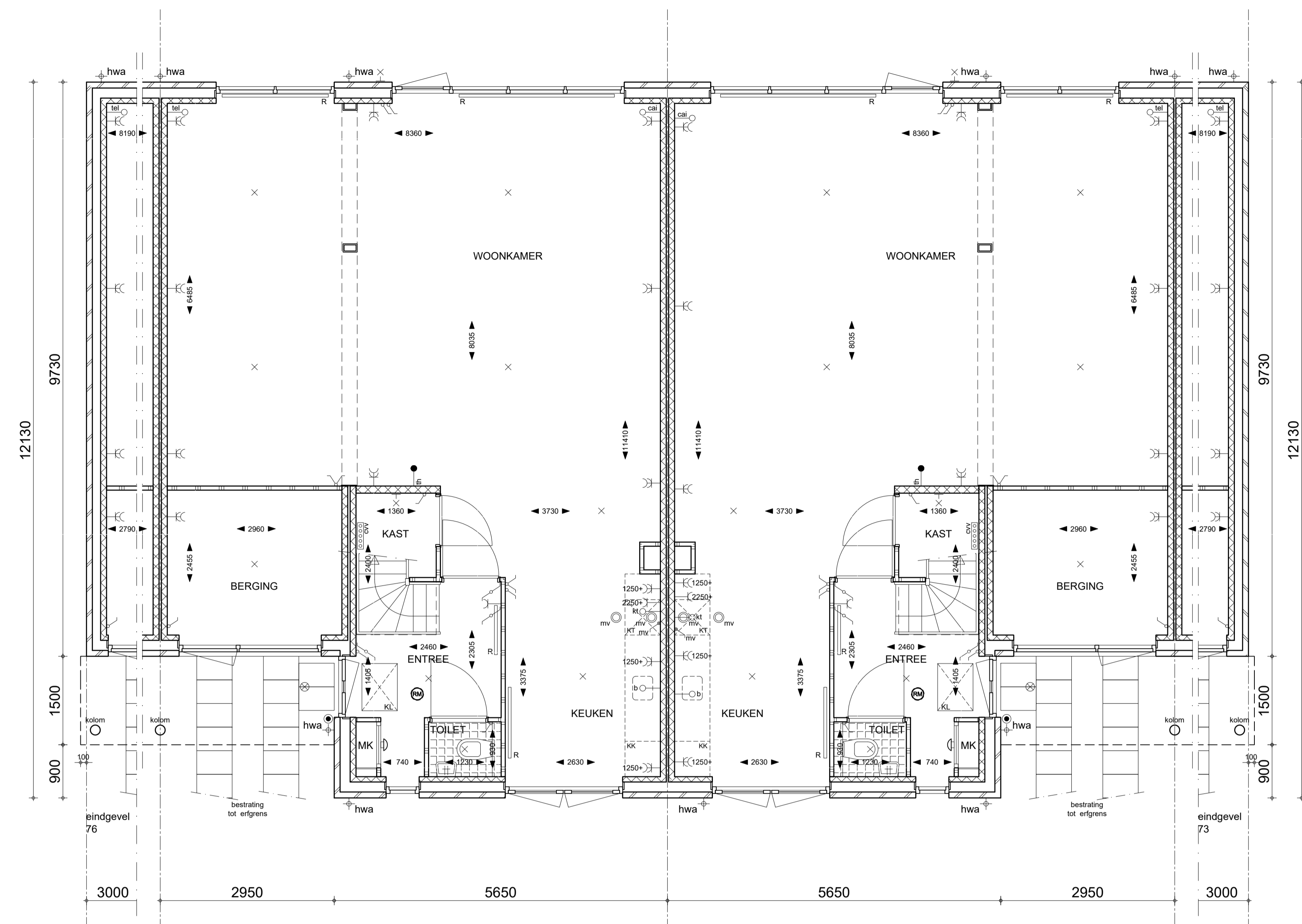
begane grond type B-basis
